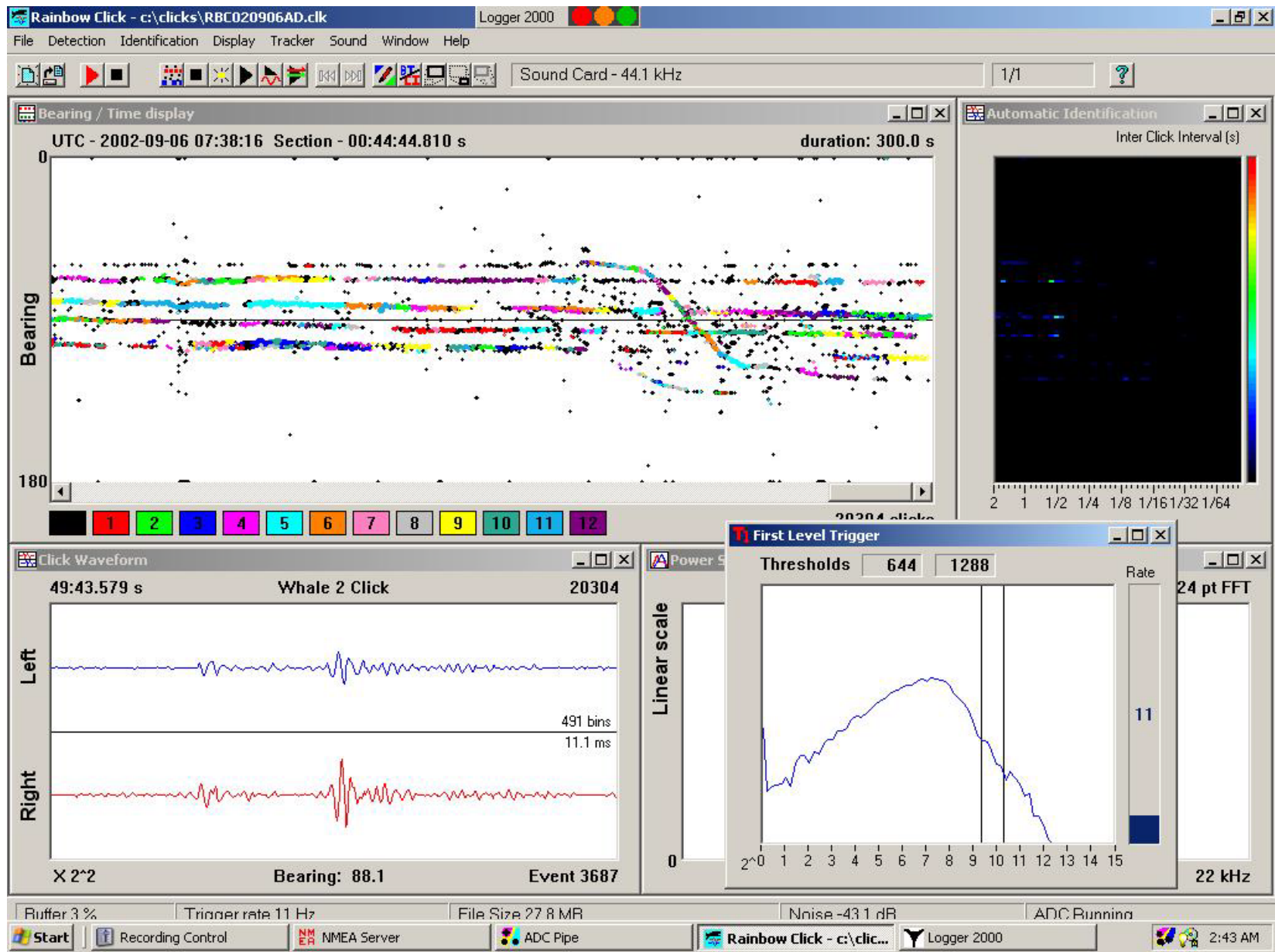
Figure 9. Screen shot from the rainbow click software package showing sperm whale and dolphin tracks.
