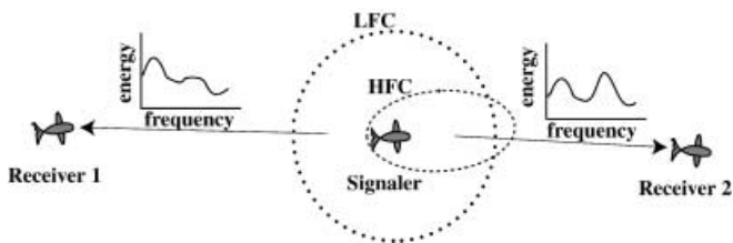
Fig. 5 Direction of movement cueing via mixed-directionality in an acoustic signal. When the signaler produces a call with mixed-directionality, energy in the low-frequency component (LFC) radiates in a fairly omni-directional fashion while the high-frequency component (HFC) is beamed forward as illustrated by the dashed ellipses around the signaler. The receiving whales can deduce the direction of movement of the signaler by the relative level of these two components in the received call. Relatively low levels of high-frequency energy will be heard by receiver 1 from whom the signaler is moving away, while higher levels of high-frequency energy in the call heard by receiver 2 indicate the signaler is oriented and moving toward it
