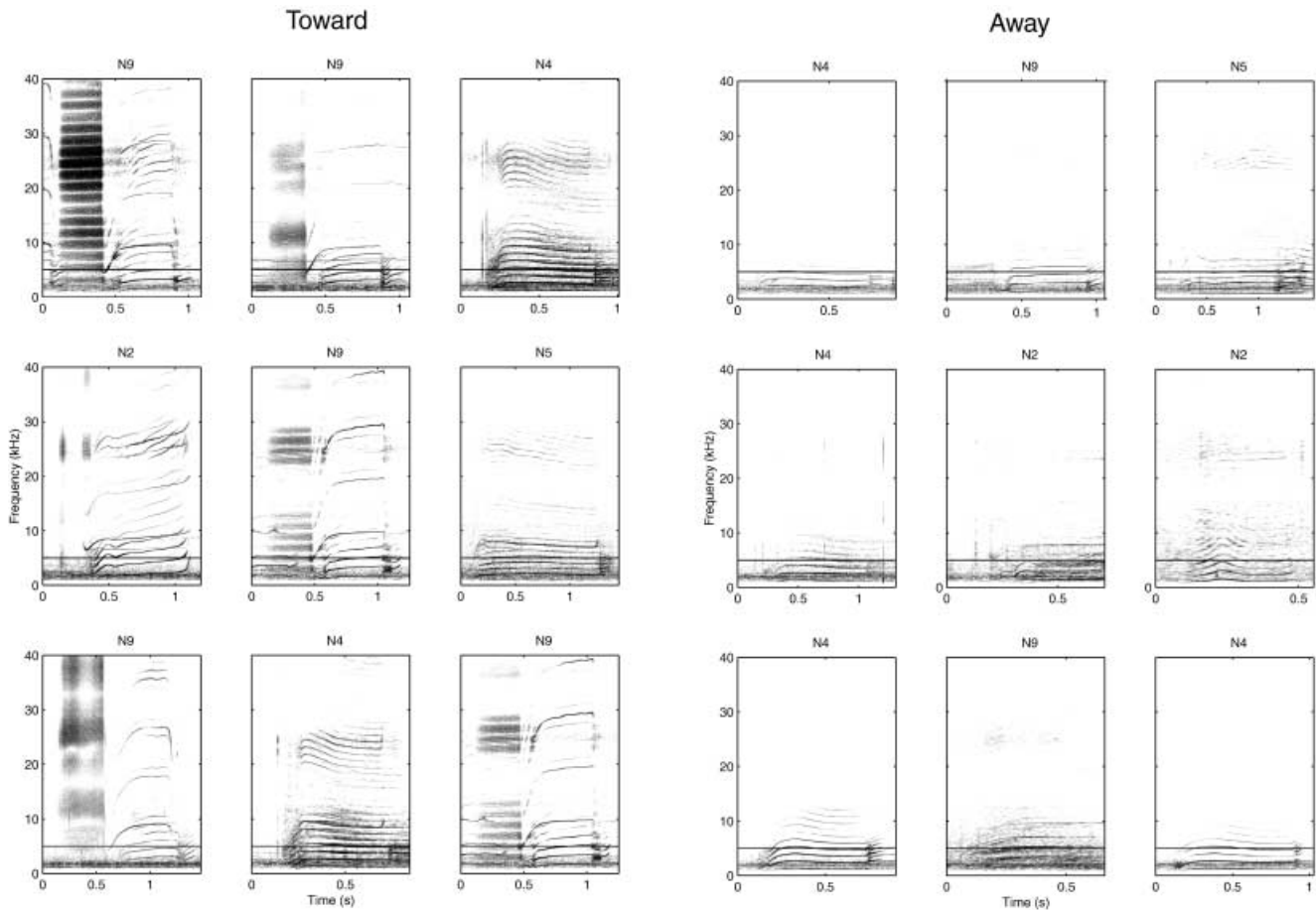
Fig. 3 Spectrograms of a random selection of calls of types that contain high-frequency components from animals moving toward ( left ) and away ( right ) from the array. The type of each call is noted above its spectrogram, and the line at 5 kHz marks the frequency below which energy was summed in the 1–5 kHz band. Note the clear differences in the spectral structure of calls depending on
